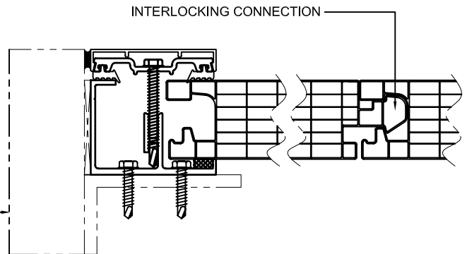
C SECTION
