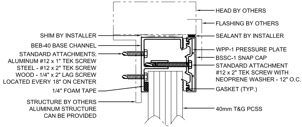
A SECTION
