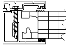
OPTIONAL SYSTEM FOR VERTICAL SPANS GREATER THAN 25 FEET
