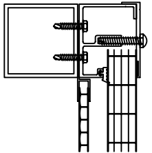
25MM SECTION
