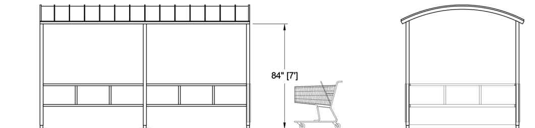
SIDE ELEVATION
