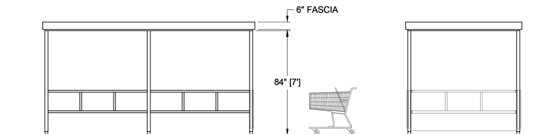
SIDE ELEVATION
