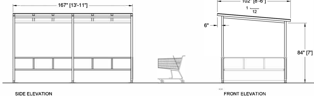
SIDE ELEVATION
