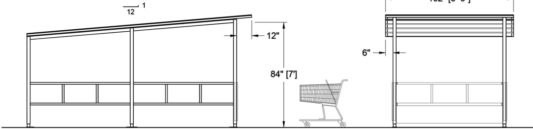
SIDE ELEVATION
