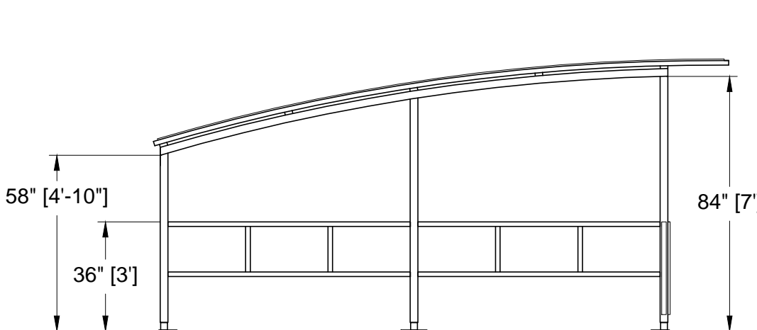
SIDE ELEVATION
