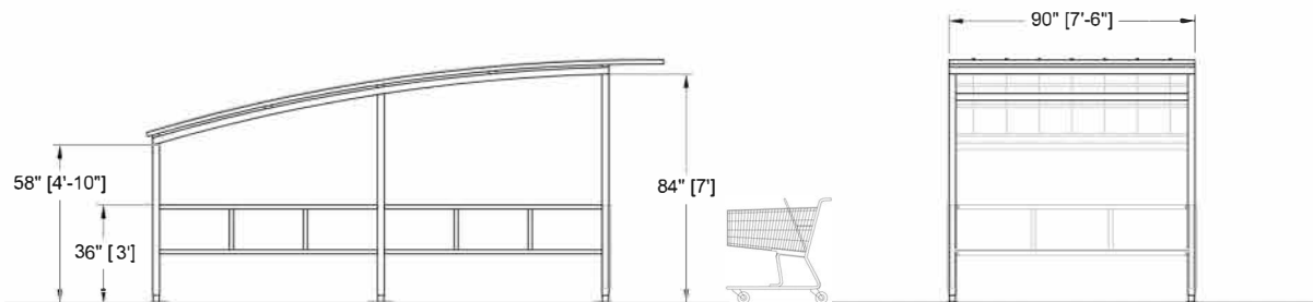
SIDE ELEVATION
