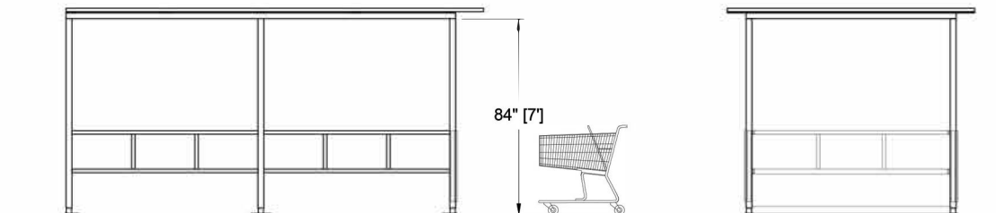
SIDE ELEVATION
