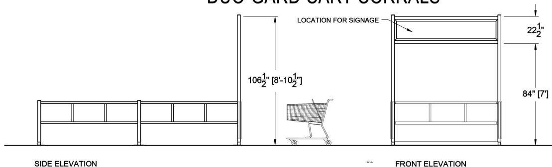
SIDE ELEVATION
