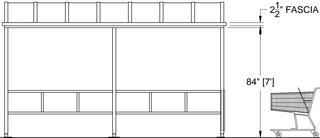
SIDE ELEVATION
