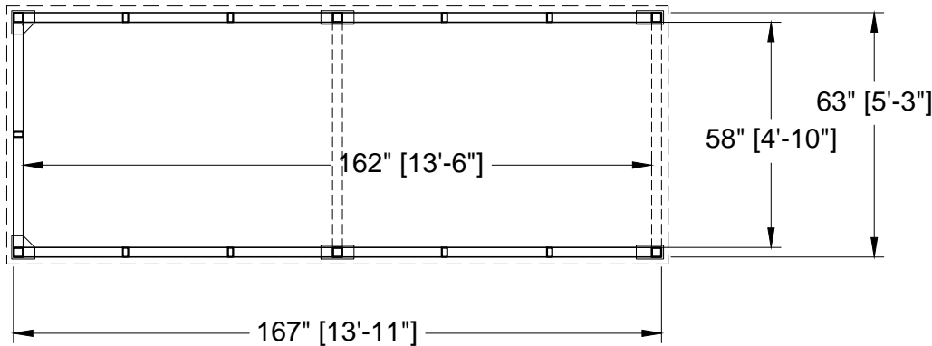
PLAN VIEW
