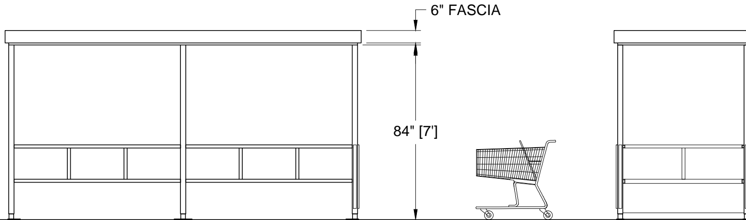
SIDE ELEVATION
