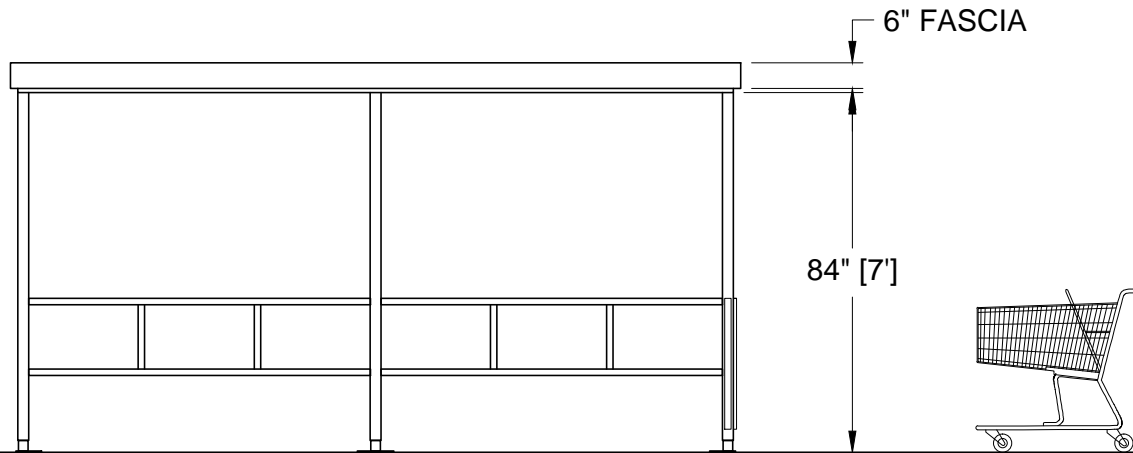
SIDE ELEVATION
