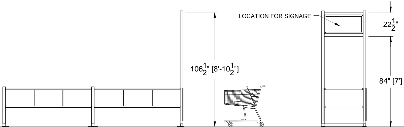
SIDE ELEVATION
