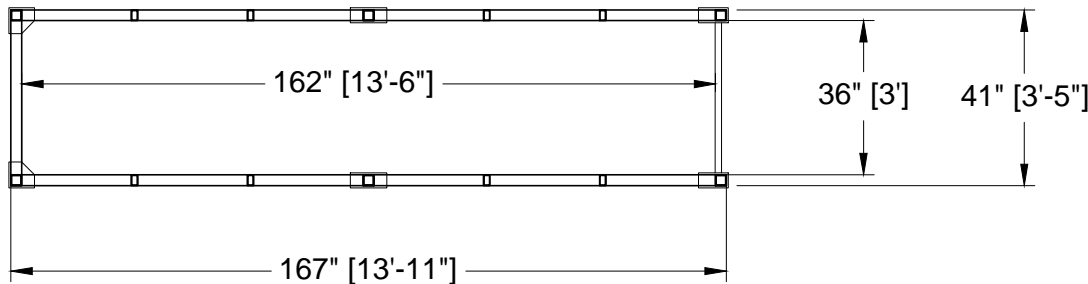
PLAN VIEW
