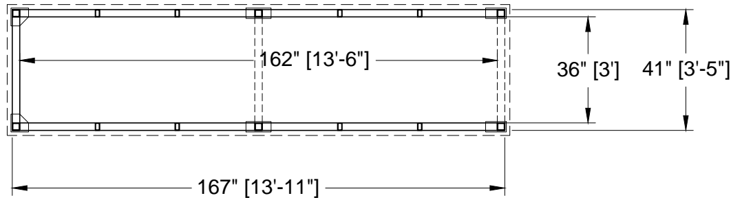
PLAN VIEW
