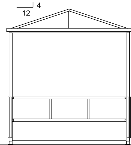
FRONT ELEVATION
